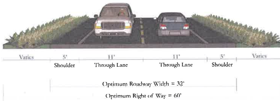
Figure I4b: Major and Minor Collector Roadway, outside an UGB
