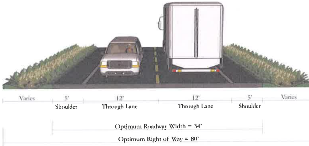
Figure I4a: Minor Arterial Roadway, outside an UGB
